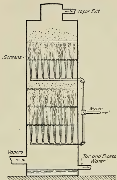
FIG. 61.—Rain Scrubber.
